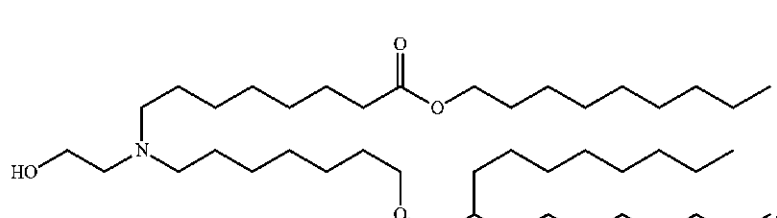
(Compound 30)
