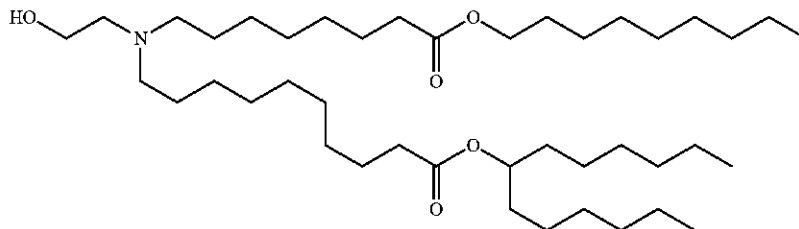
Chemical Formula: C 42 H 83 NO 5 Molecular Weight: 682.128
