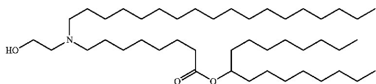
(Compound 1)
