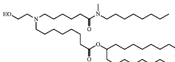
Chemical Formula: C 42 H 84 N 2 O 4 Molecular Weight: 681.144
