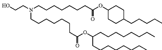
Chemical Formula: C 46 H 89 NO 5 Molecular Weight: 736.220
