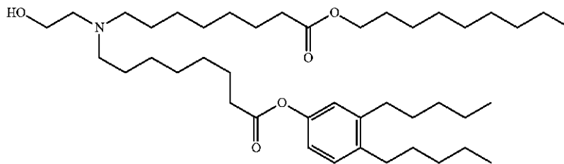
3,4-Dipentylphenyl 8-((2-hydroxyethyl)(8-(nonyloxy)-8-oxooctyl)amino)octanoate
