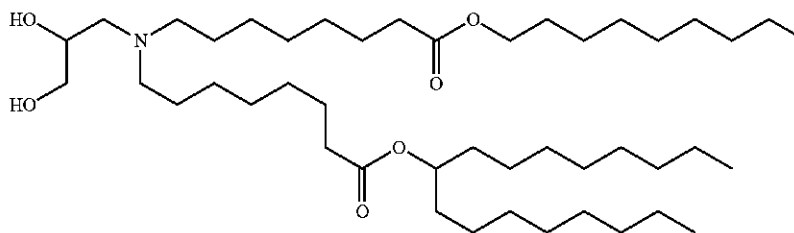
Chemical Formula: C 45 H 89 NO 6 Molecular Weight: 740.21
