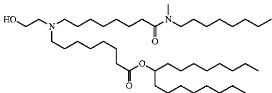
Chemical Formula: C 44 H 88 N 2 O 4 Molecular Weight: 709.198
