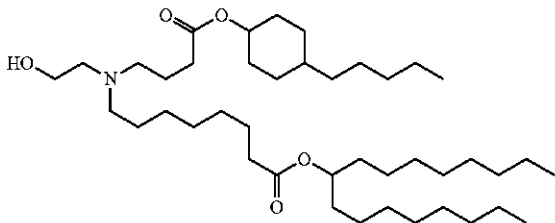
Chemical Formula: C 42 H 81 NO 5 Molecular Weight: 680.112
