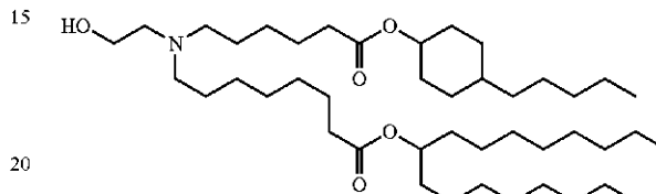
Chemical Formula: C 44 H 85 NO 5 Molecular Weight: 708.166
