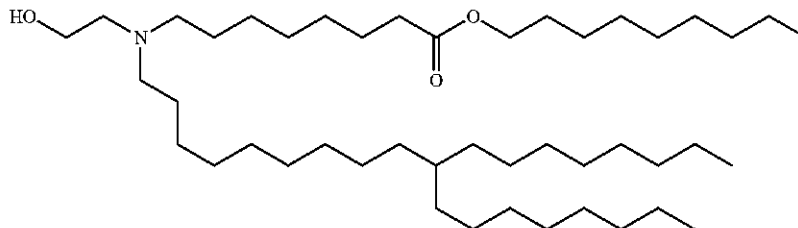
XX53. Compound 153: Nonyl 8-((2-hydroxyethyl)(10-octyloctadecyl)amino)octanoate
