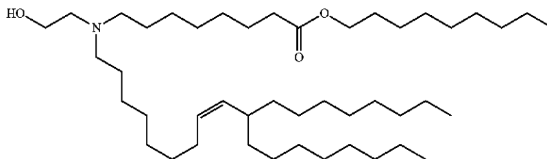
Nonyl (Z)-8-((2-hydroxyethyl)(10-octyloctadec-8-en-1-yl)amino)octanoate
