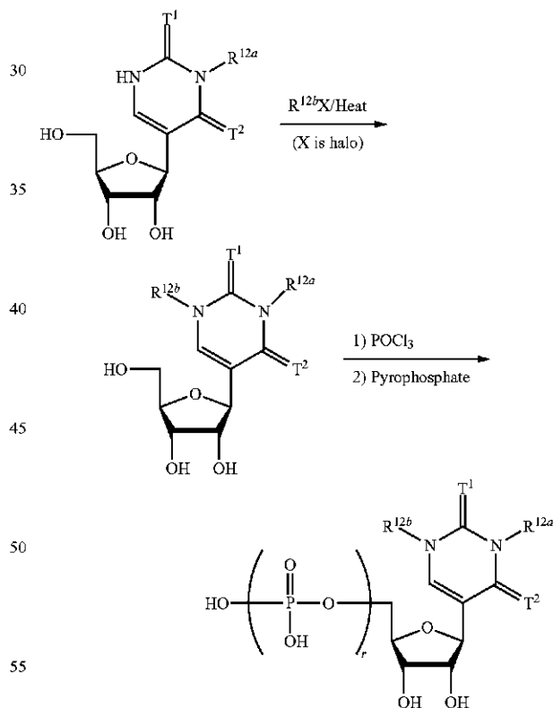
Scheme 11
