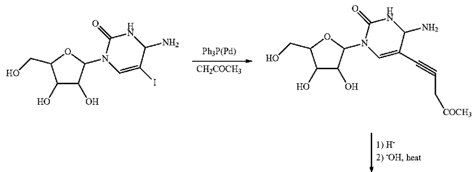
Scheme 9
