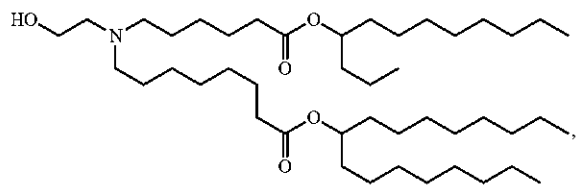
(Compound 78)
