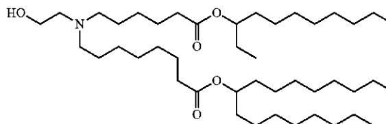
Chemical Formula: C_{44}H_{87}NO_5 Molecular Weight: 710.18
