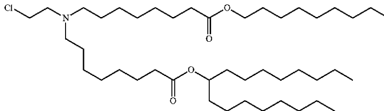
Heptadecan-9-yl 8-((2-chloroethyl)(8-(nonyloxy)-8-oxooctyl)amino)octanoate
