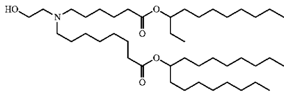
(Compound 77)
