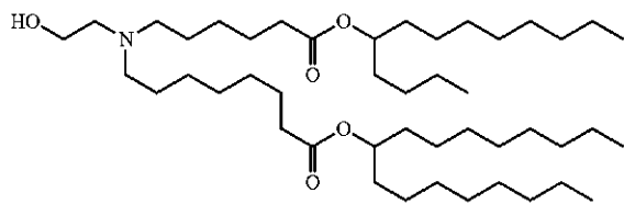
(Compound 79)
