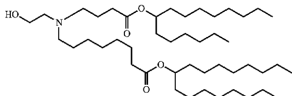
(Compound 75)
