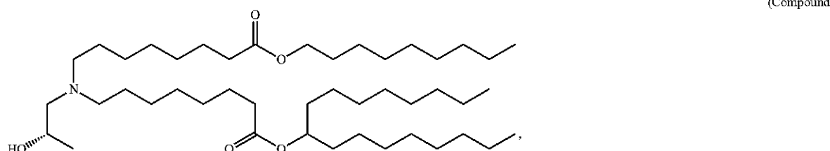
(Compound 12)
