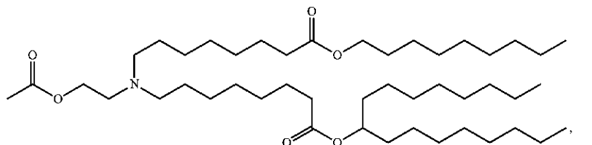
(Compound 10)
