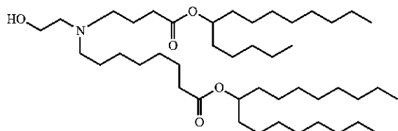
(Compound 73)
