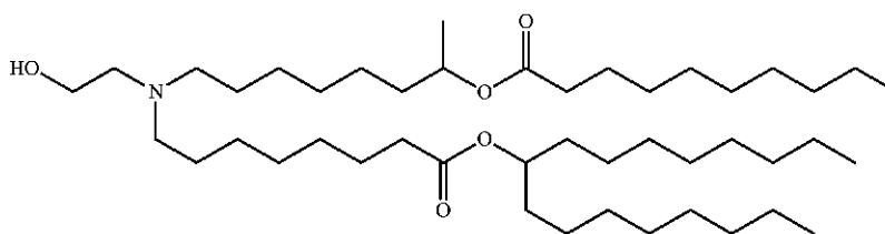
8-((8-(Heptadecan-9-yloxy)-8-oxooctyl)(2-hydroxyethyl)amino)octan-2-yl decanoate
